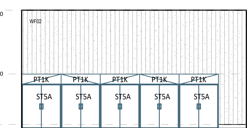
3 ELEVATION DETAIL 1 : 50
