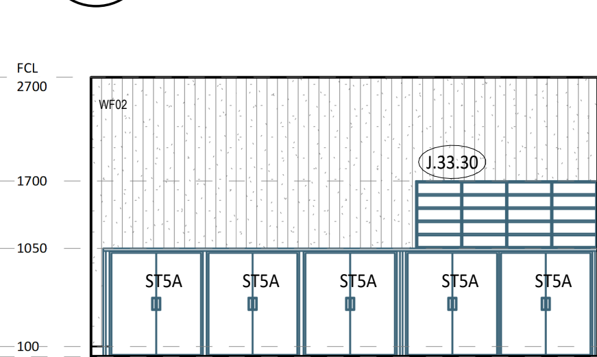
5 ELEVATION DETAIL 1 : 50
