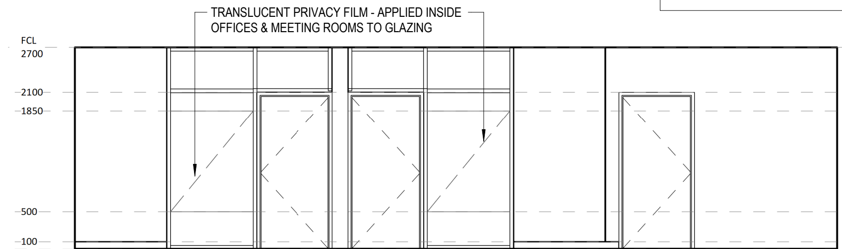
10 ELEVATION DETAIL 1 : 50
