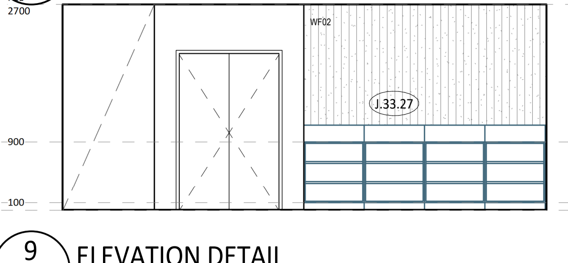
9 ELEVATION DETAIL 1 : 50
