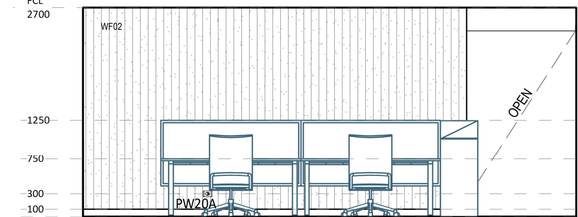
8 ELEVATION DETAIL 1 : 50
